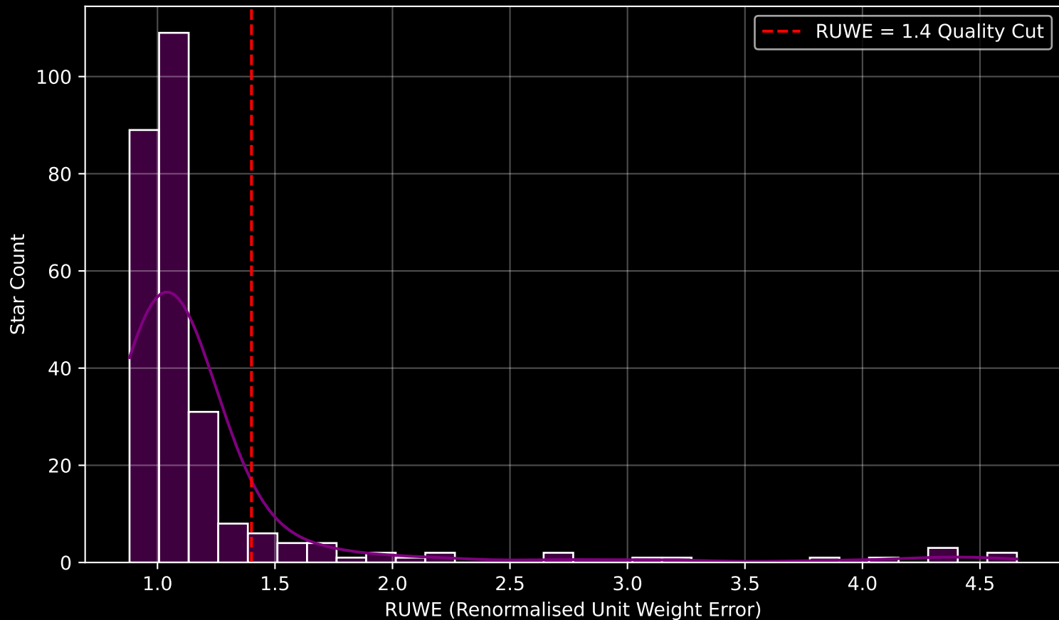
GALAH DR4 Field [466] RUWE Distribution (n= 268)
