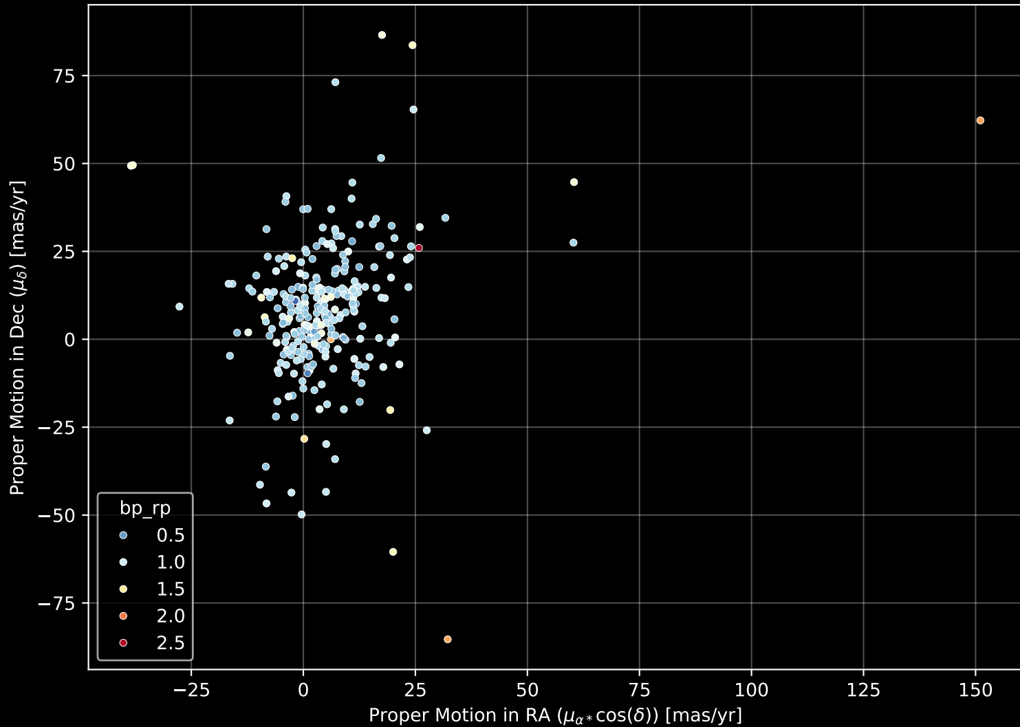
GALAH DR4 Field: [466] Proper Motion Diagram (n= 280)
