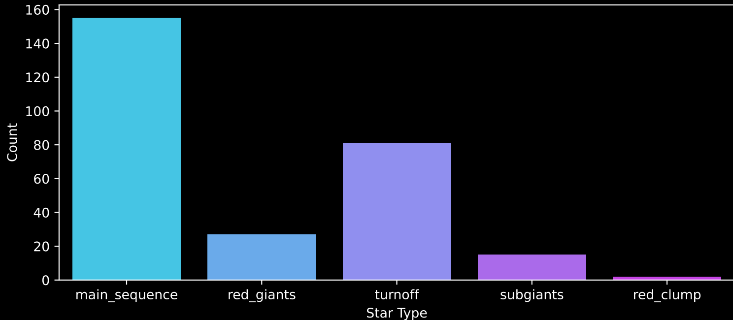
GALAH DR4 Field: [466] Count plot of Star Type
